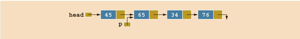
FIGURE 16-10 Node to be deleted is with info 34
