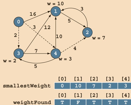
FIGURE 20-11 Graph after the third iteration of Steps 3 to 5
