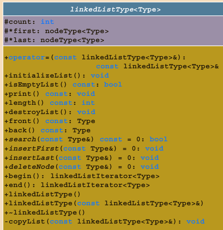
FIGURE 16-20 UML class diagram of the class linkedListType
