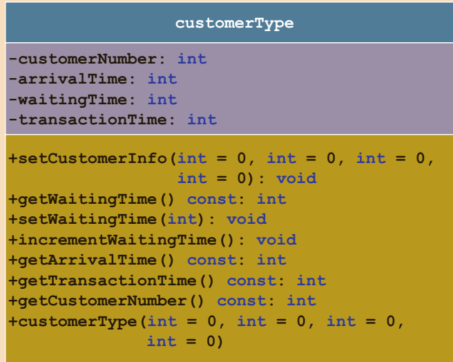
FIGURE 17-36 UML class diagram of the class customerType
