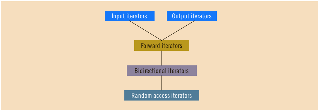
FIGURE 21-1 Iterator hierarchy
