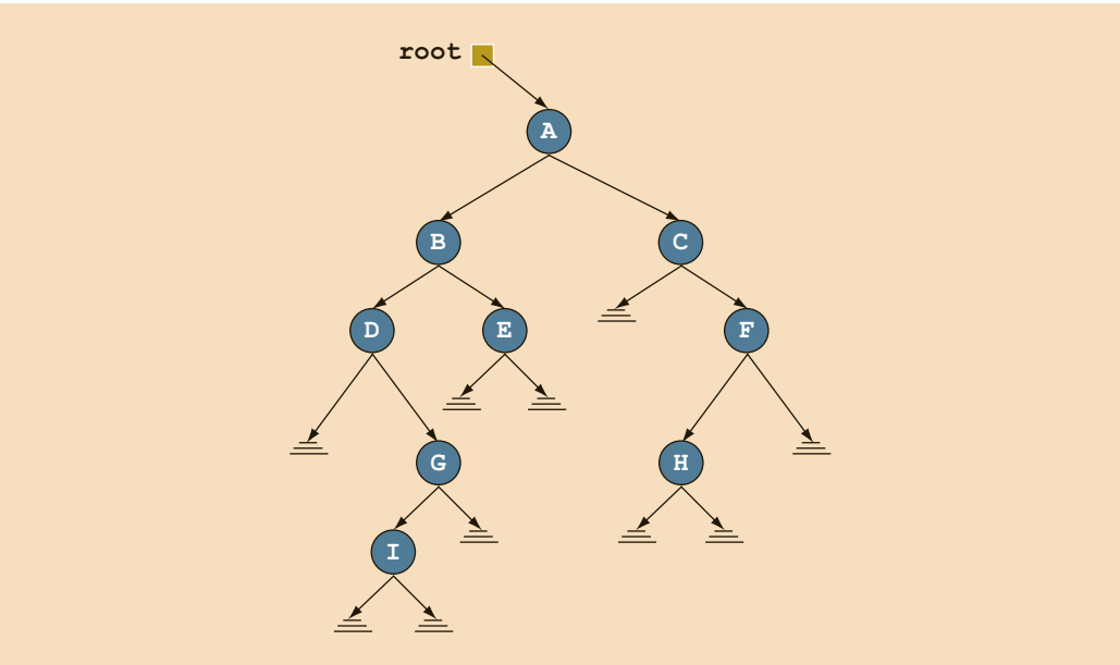
FIGURE 19-5 Binary tree
