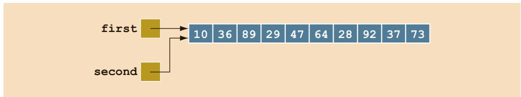
FIGURE 12-10 first and second after the statement second = first; executes
