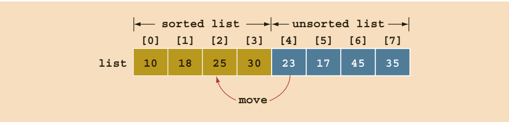
FIGURE 18-13 Move list[4] into list[2]
