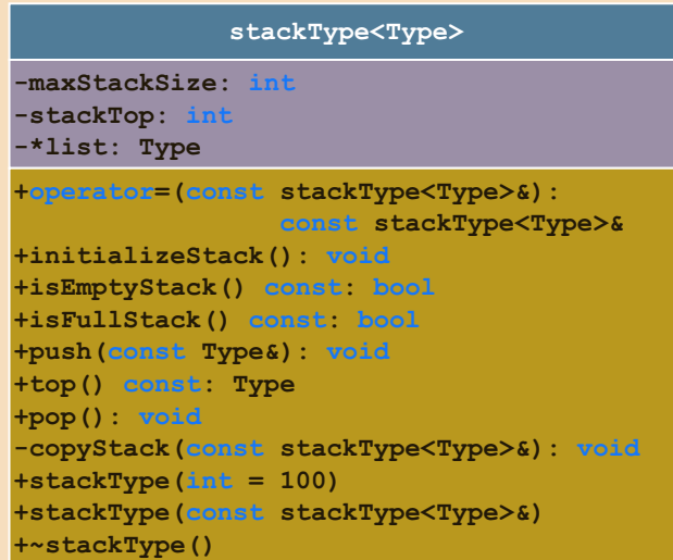
FIGURE 17-5 UML class diagram of the class stackType
