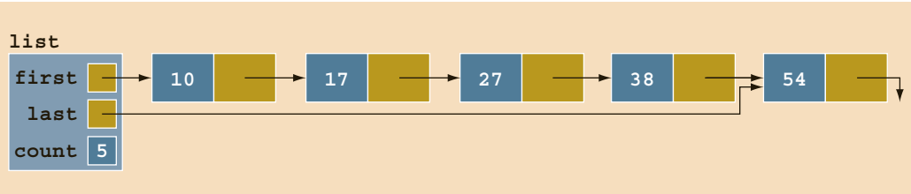
FIGURE 16-32 list after inserting 10
