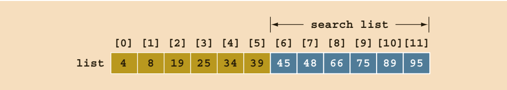
FIGURE 18-3 Search list, list[6] ... list[11]
