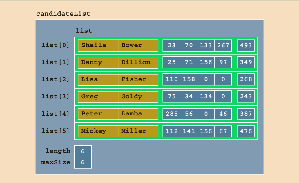
FIGURE 18-48 candidateList after a call to the function addVotes
