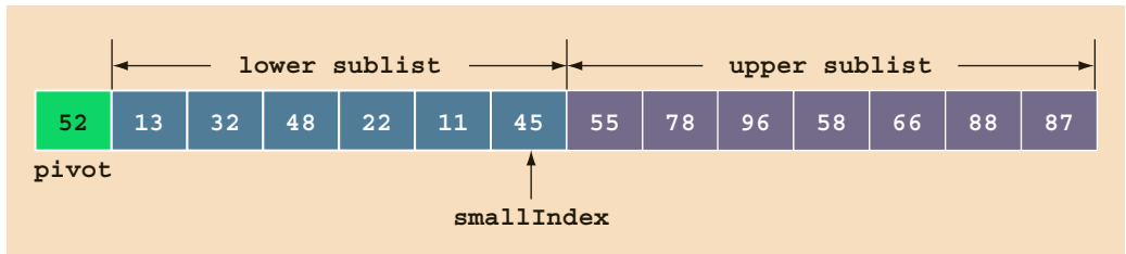
FIGURE 18-28 List elements after arranging into the lower sublist and upper sublist
