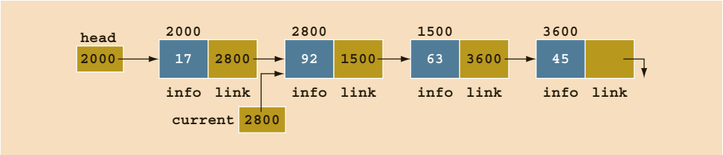
FIGURE 16-6 List after the statement current = current->link; executes
