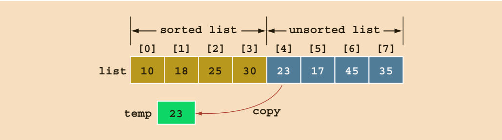
FIGURE 18-14 Copy list[4] into temp
