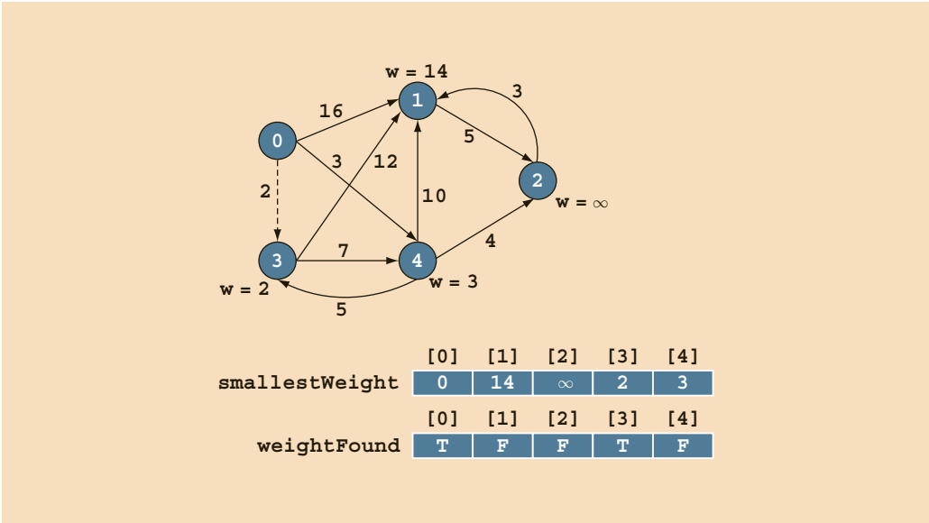
FIGURE 20-9 Graph after the first iteration of Steps 3 to 5
