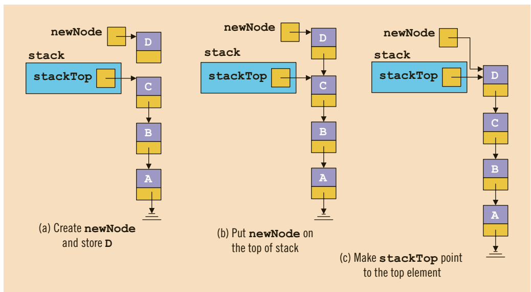
FIGURE 17-14 Push operation
