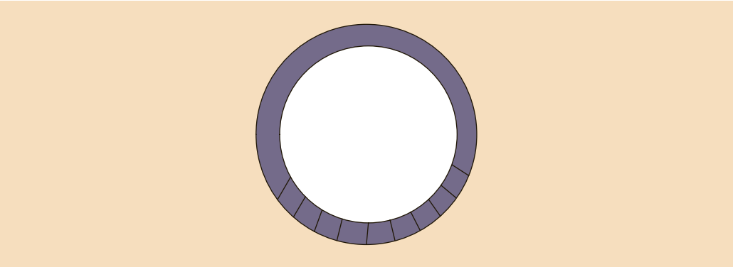
FIGURE 17-30 Circular queue
