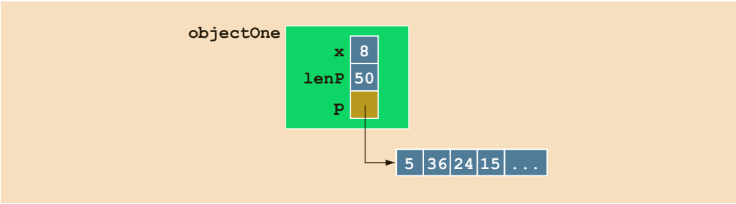
FIGURE 12-19 Object objectOne
