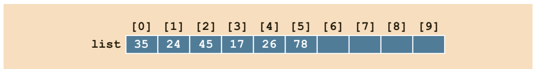
FIGURE 12-23 Array list
