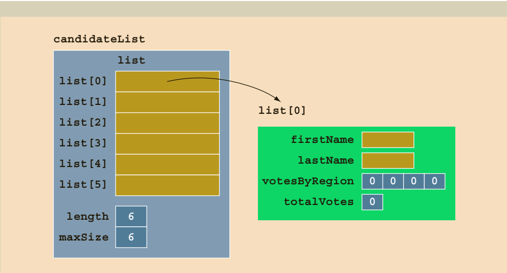
FIGURE 18-40 candidateList
