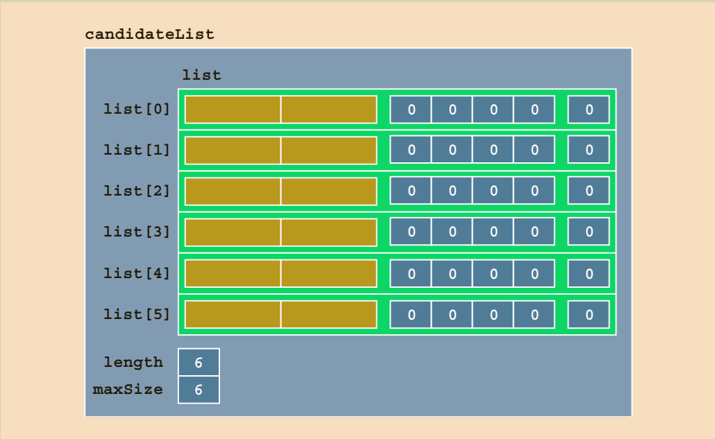
FIGURE 18-41 candidateList
