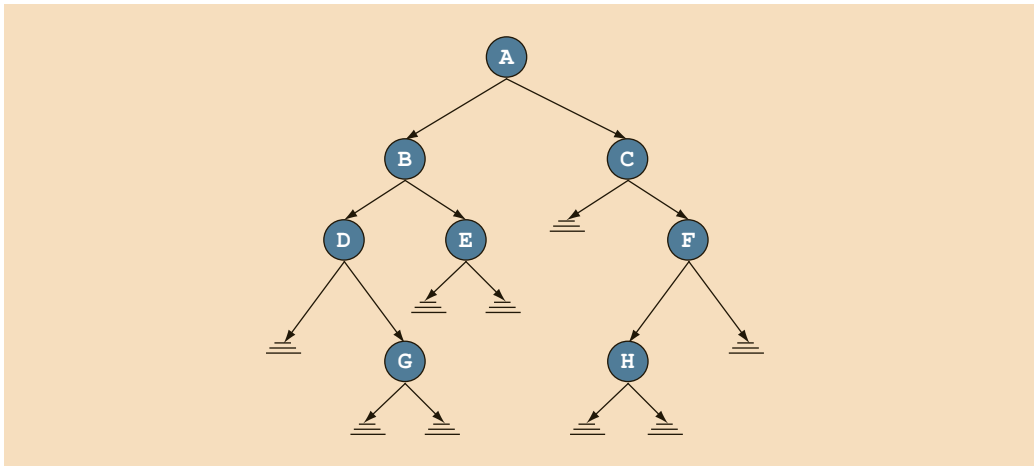
FIGURE 19-1 Binary tree
