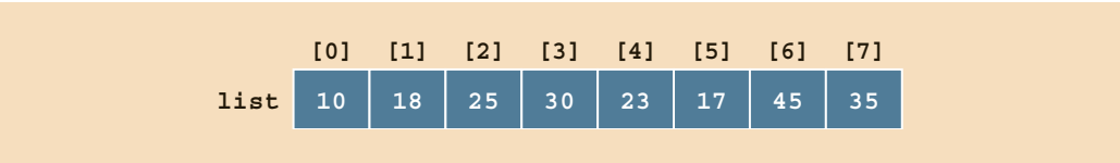
FIGURE 18-11 list
