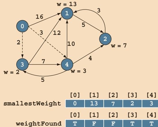
FIGURE 20-10 Graph after the second iteration of Steps 3 to 5
