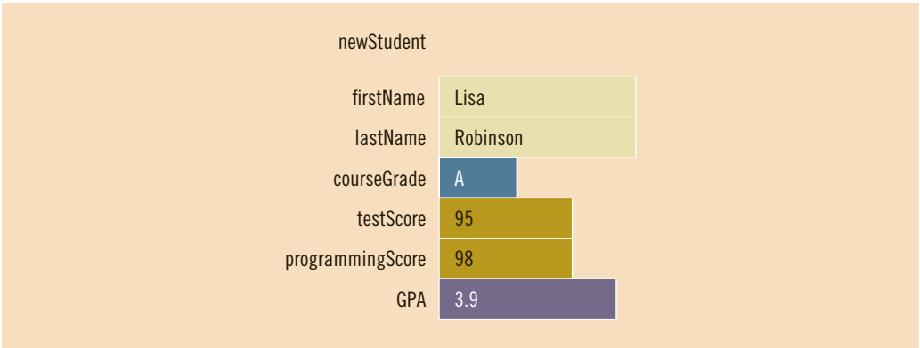
FIGURE 9-3 struct newStudent
