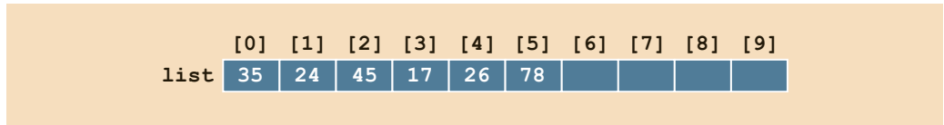
FIGURE 12-24 Array list
