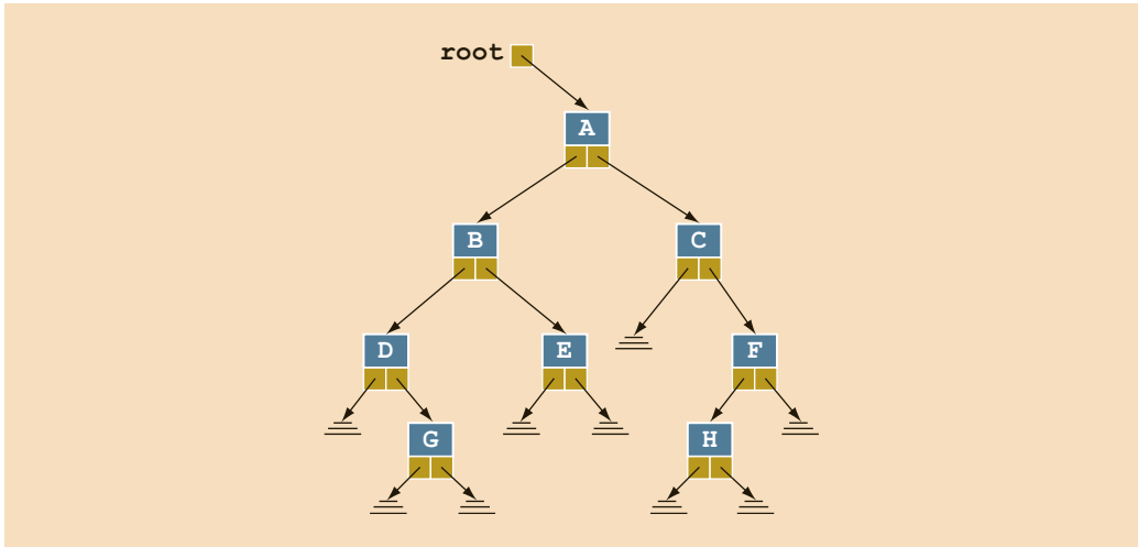
FIGURE 19-4 Binary tree
