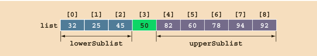
FIGURE 18-20 list after the partition
