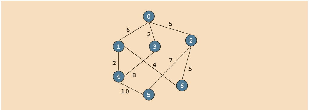
FIGURE 20-15 Weighted graph G
