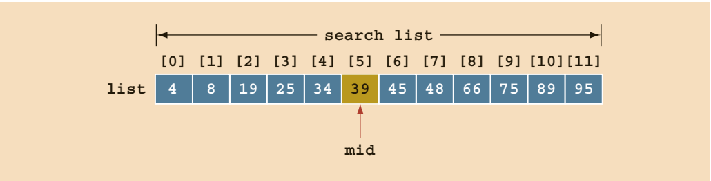
FIGURE 18-2 Search list, list[0] ... list[11]
